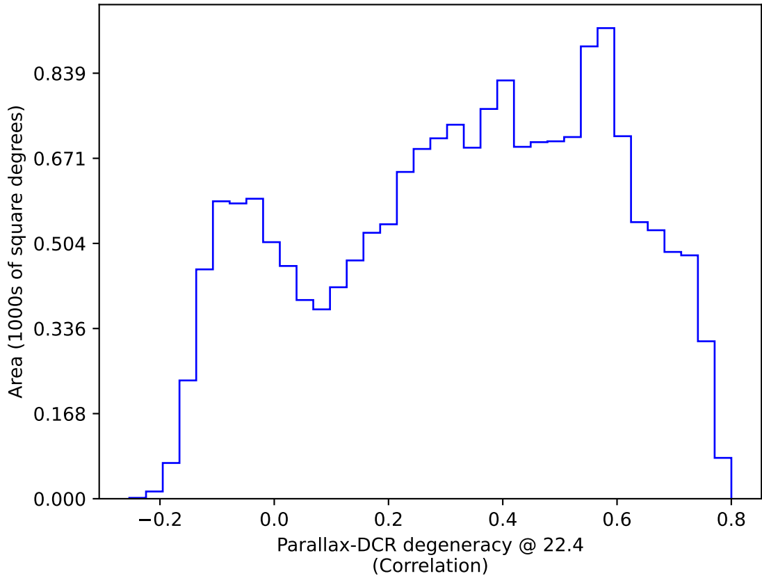
noroll_mjdp365_v3.4_10yrs WFD: Parallax-DCR degeneracy @ 22.4
