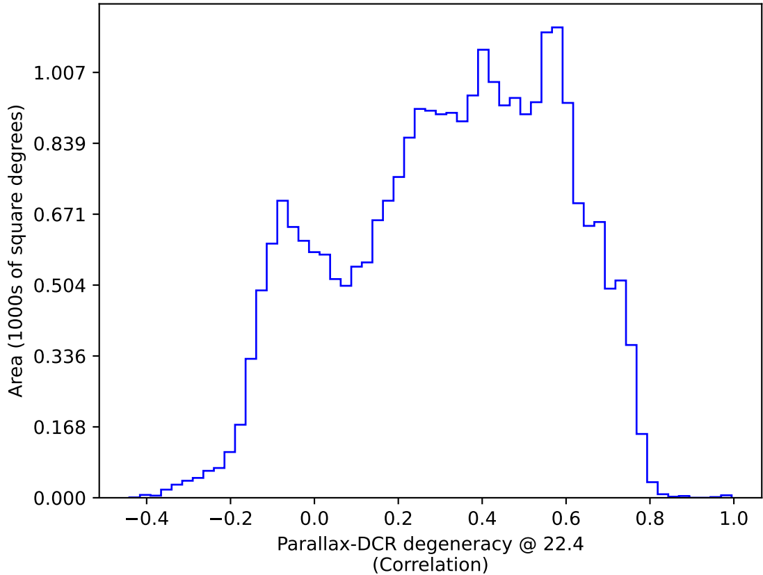
noroll_mjdp365_v3.4_10yrs All sky: Parallax-DCR degeneracy @ 22.4
