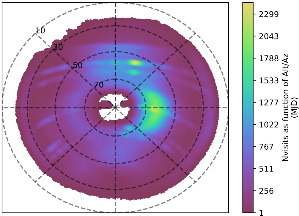
noroll_mjdp365_v3.4_10yrs z band: Nvisits as function of Alt/Az
