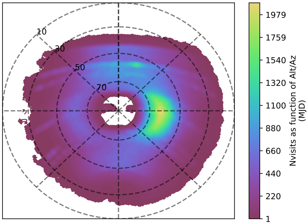
noroll_mjdp365_v3.4_10yrs y band: Nvisits as function of Alt/Az
