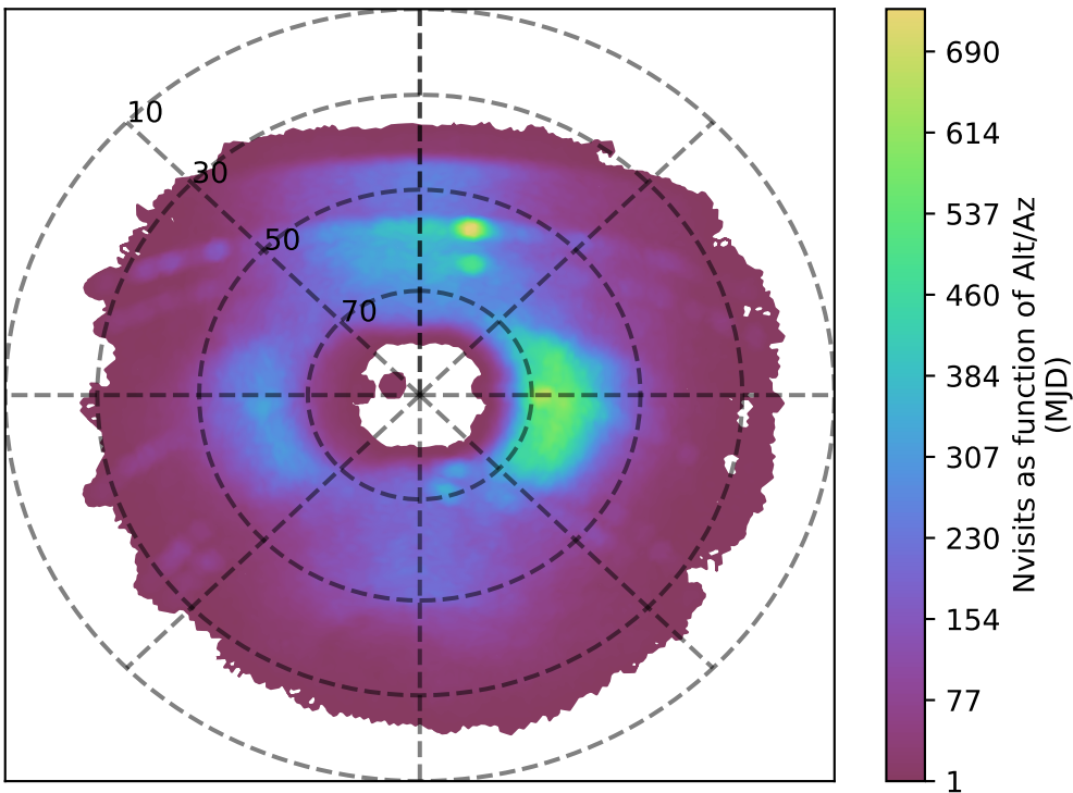
noroll_mjdp365_v3.4_10yrs u band: Nvisits as function of Alt/Az
