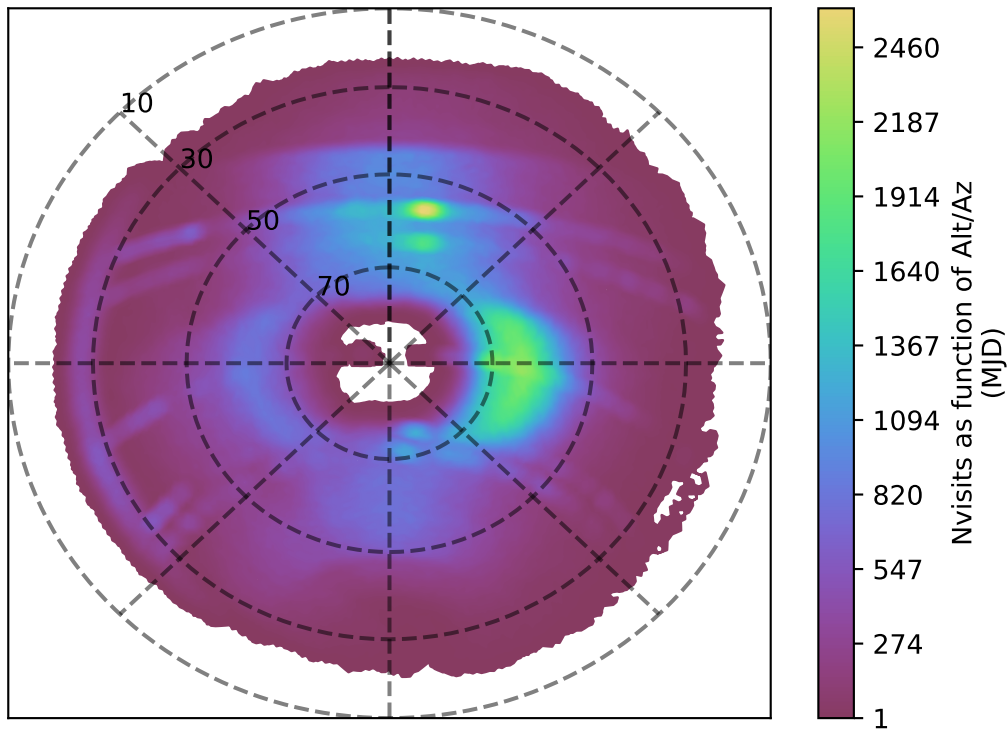
noroll_mjdp365_v3.4_10yrs r band: Nvisits as function of Alt/Az
