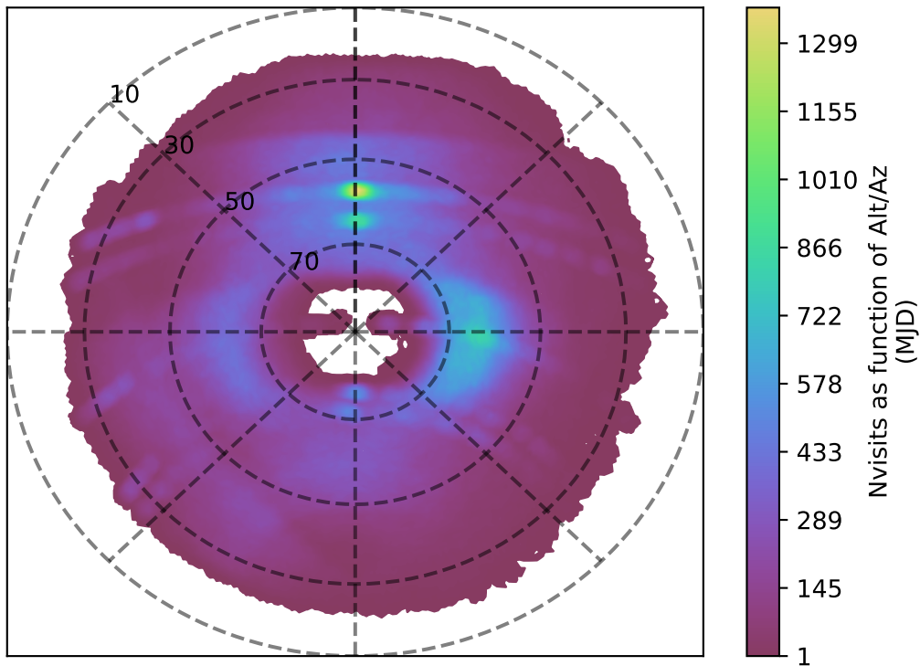
noroll_mjdp365_v3.4_10yrs g band: Nvisits as function of Alt/Az
