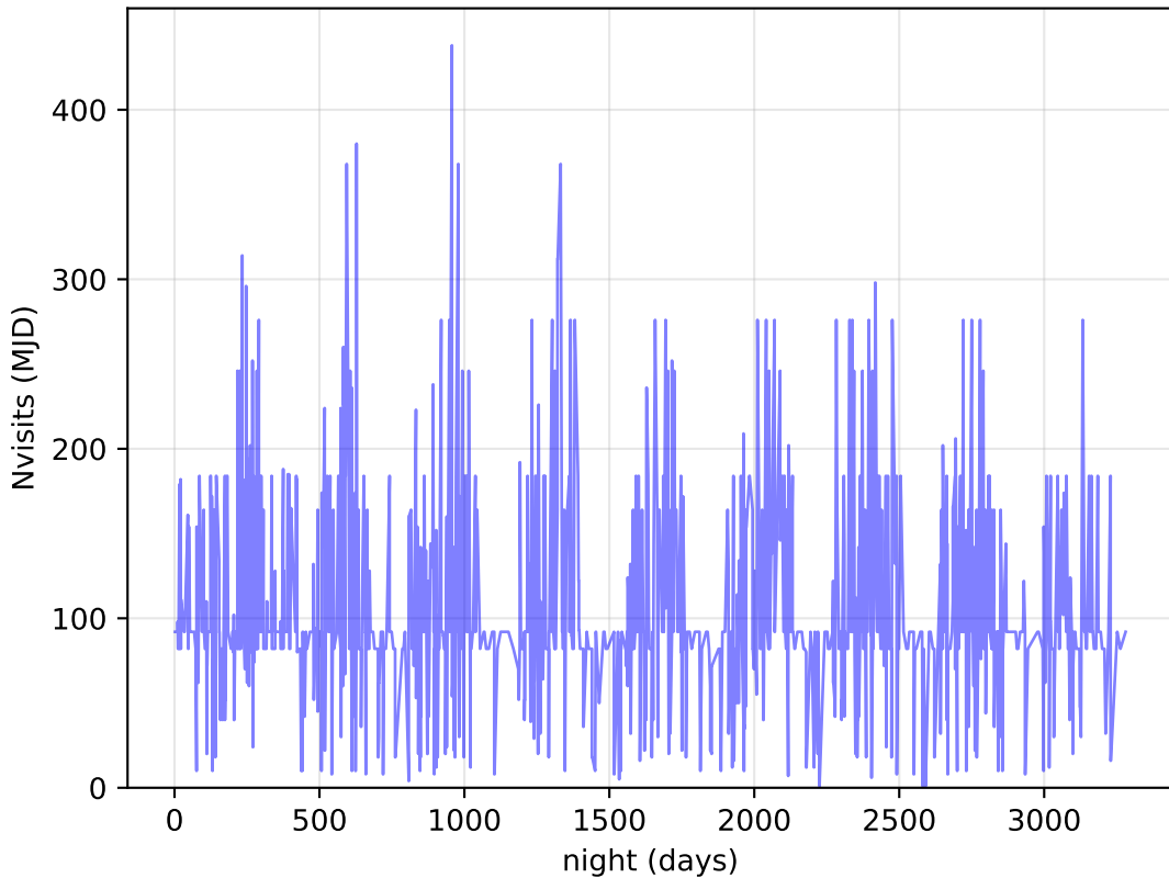
noroll_mjdp365_v3.4_10yrs DDF: Nvisits
