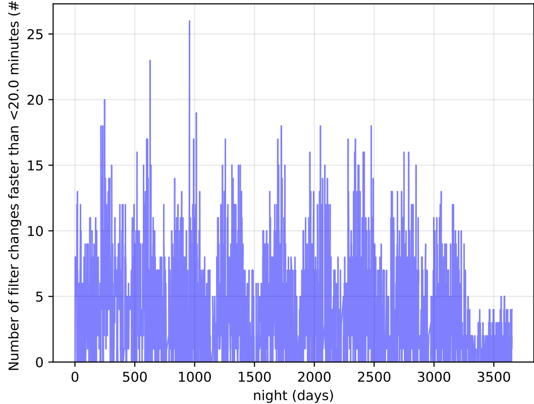
noroll_mjdp365_v3.4_10yrs Per Night: Number of filter changes faster than <20.0 minutes
