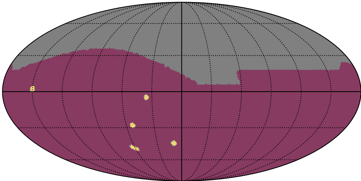
noroll_mjdp365_v3.4_10yrs All sky: NumberOfQuickRevisits
