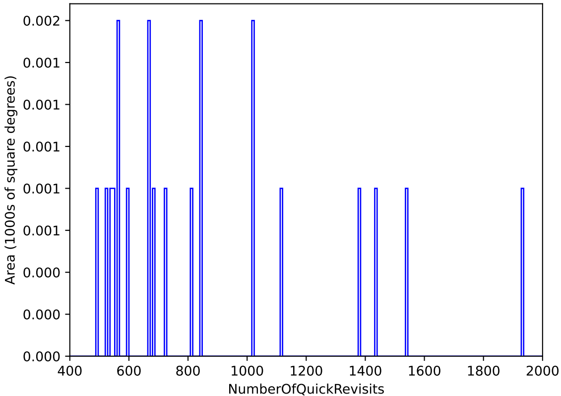
noroll_mjdp365_v3.4_10yrs All sky: NumberOfQuickRevisits
