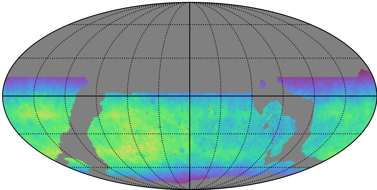
noroll_mjdp365_v3.4_10yrs WFD y band: Normalized Teff
