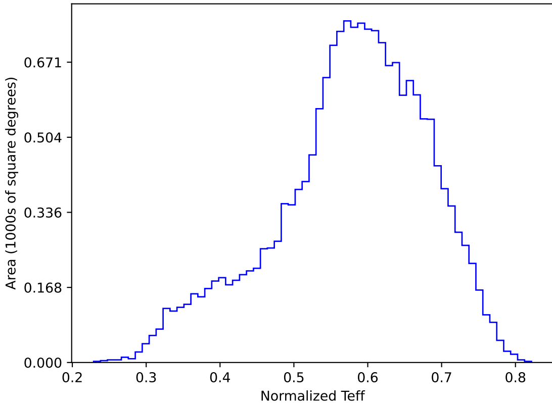
noroll_mjdp365_v3.4_10yrs WFD y band: Normalized Teff
