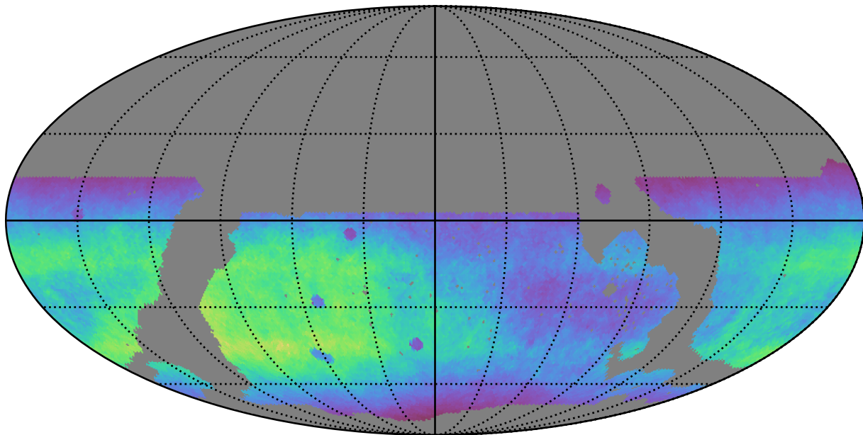
noroll_mjdp365_v3.4_10yrs WFD r band: Normalized Teff
