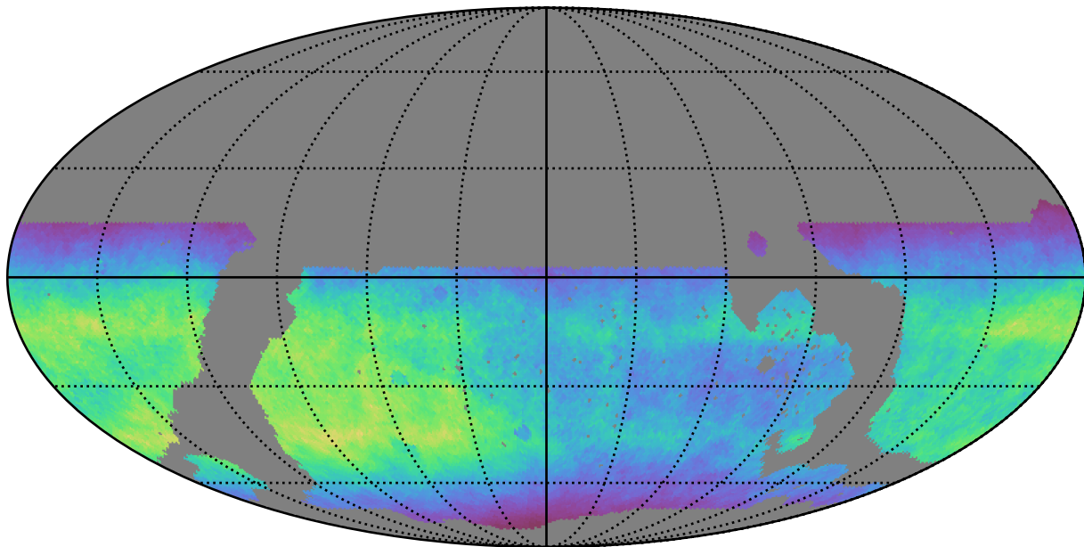
noroll_mjdp365_v3.4_10yrs WFD i band: Normalized Teff
