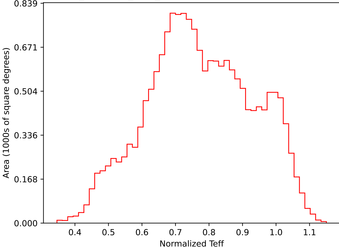
noroll_mjdp365_v3.4_10yrs WFD i band: Normalized Teff
