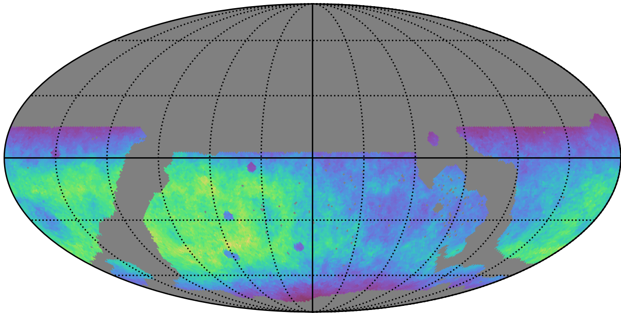
noroll_mjdp365_v3.4_10yrs WFD g band: Normalized Teff
