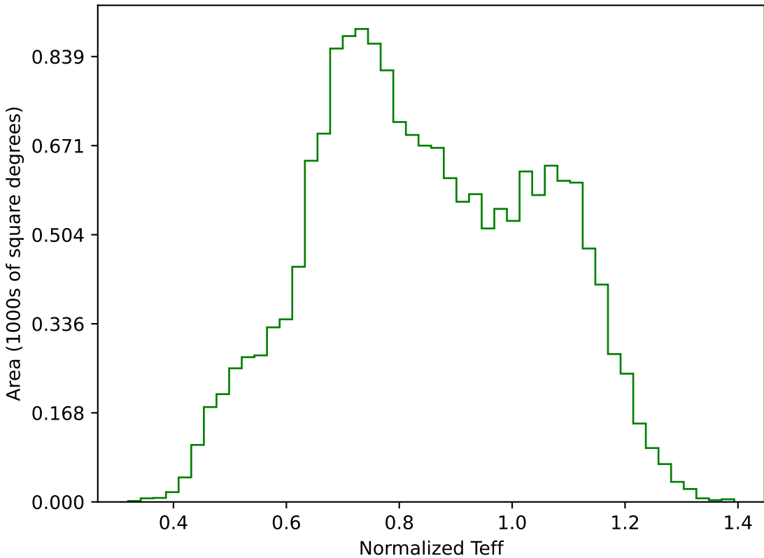
noroll_mjdp365_v3.4_10yrs WFD g band: Normalized Teff
