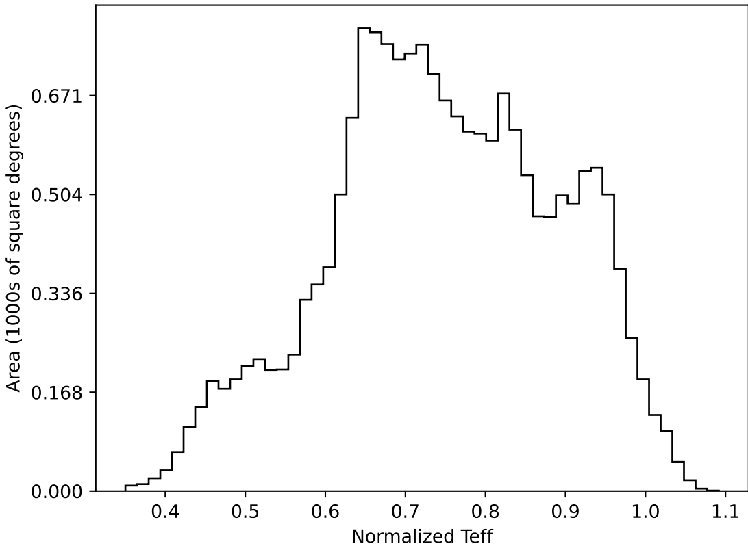
noroll_mjdp365_v3.4_10yrs WFD all bands: Normalized Teff
