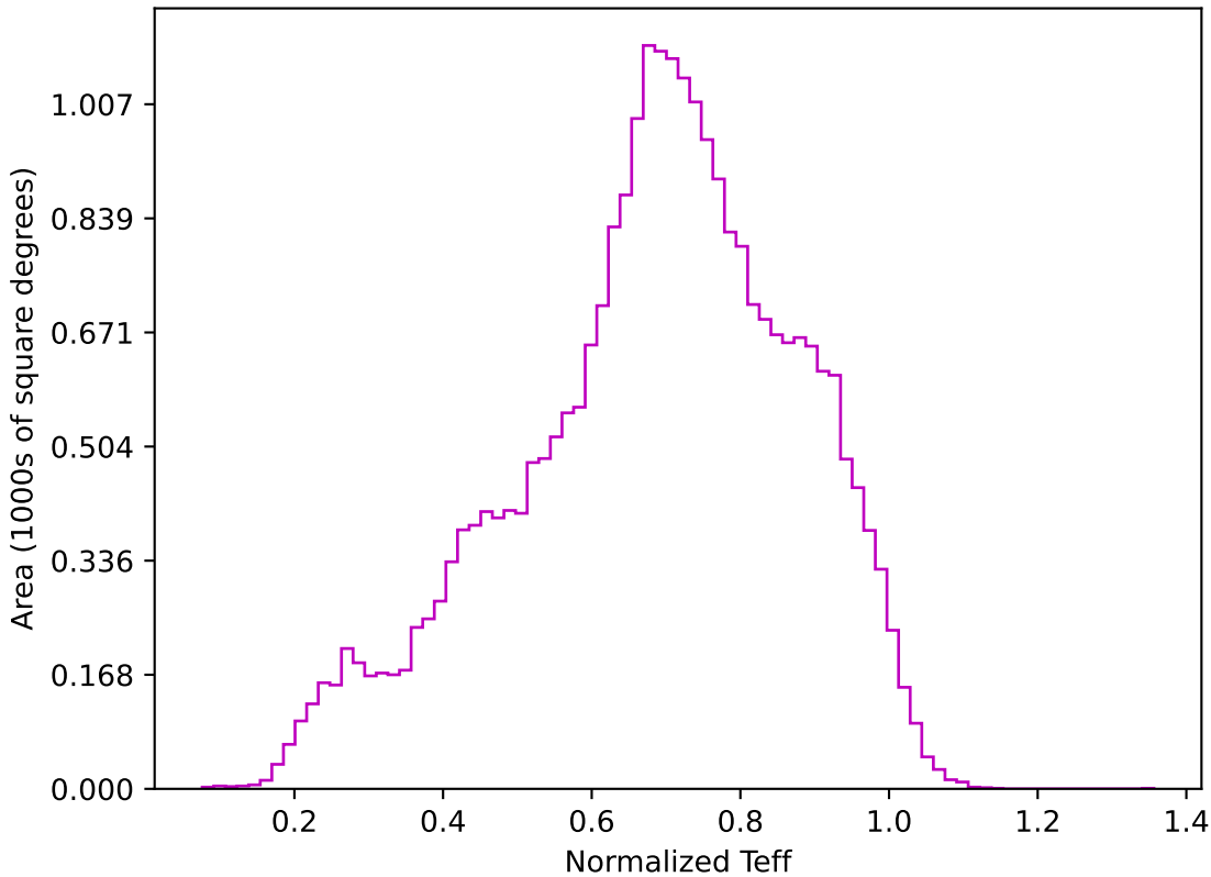
noroll_mjdp365_v3.4_10yrs All sky z band: Normalized Teff
