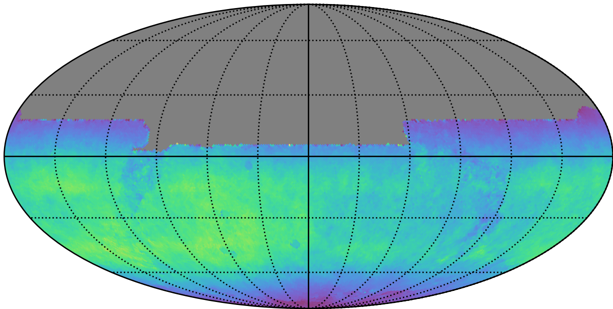
noroll_mjdp365_v3.4_10yrs All sky y band: Normalized Teff
