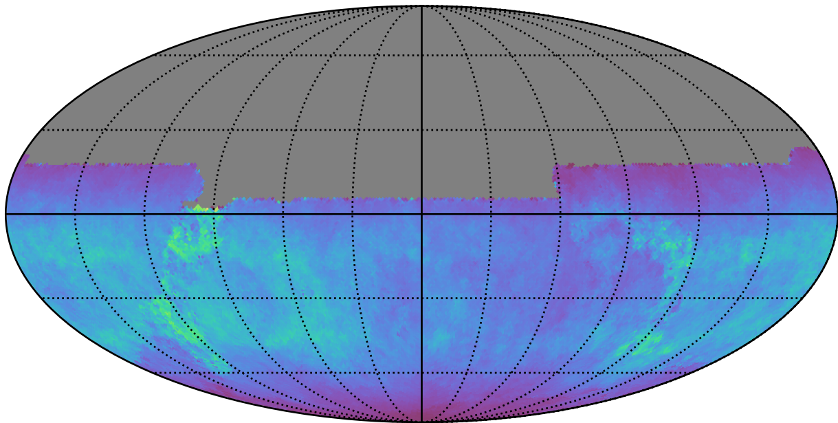
noroll_mjdp365_v3.4_10yrs All sky u band: Normalized Teff
