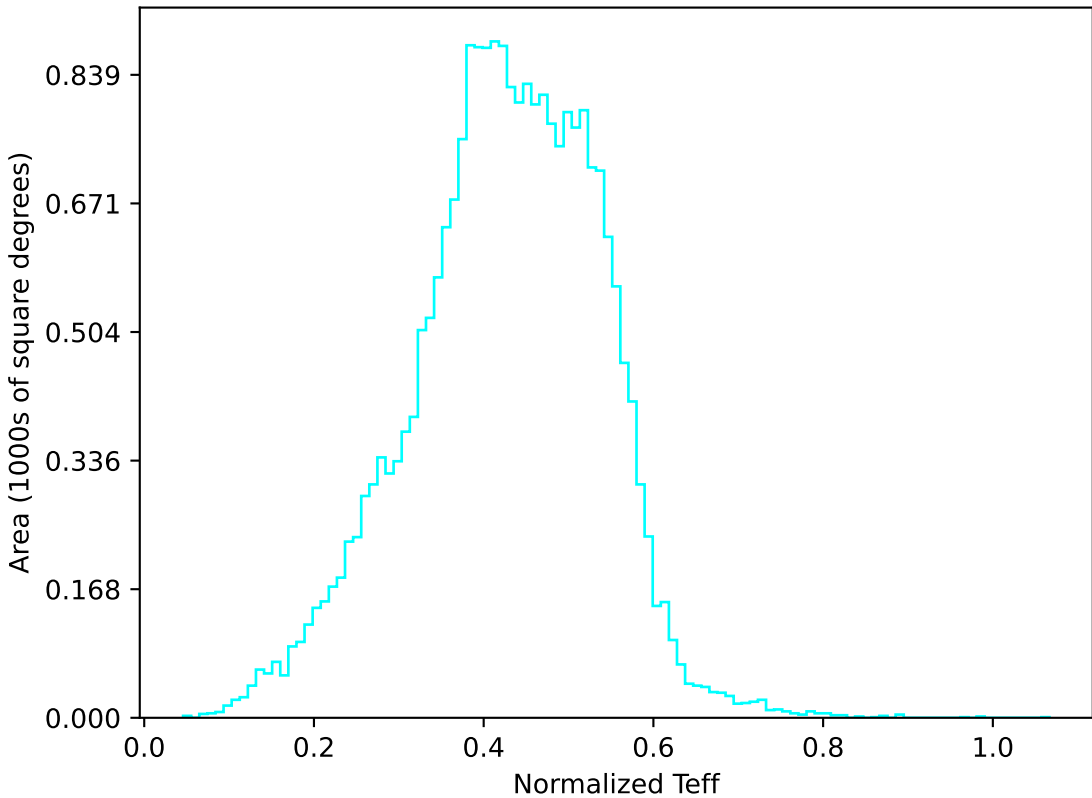
noroll_mjdp365_v3.4_10yrs All sky u band: Normalized Teff
