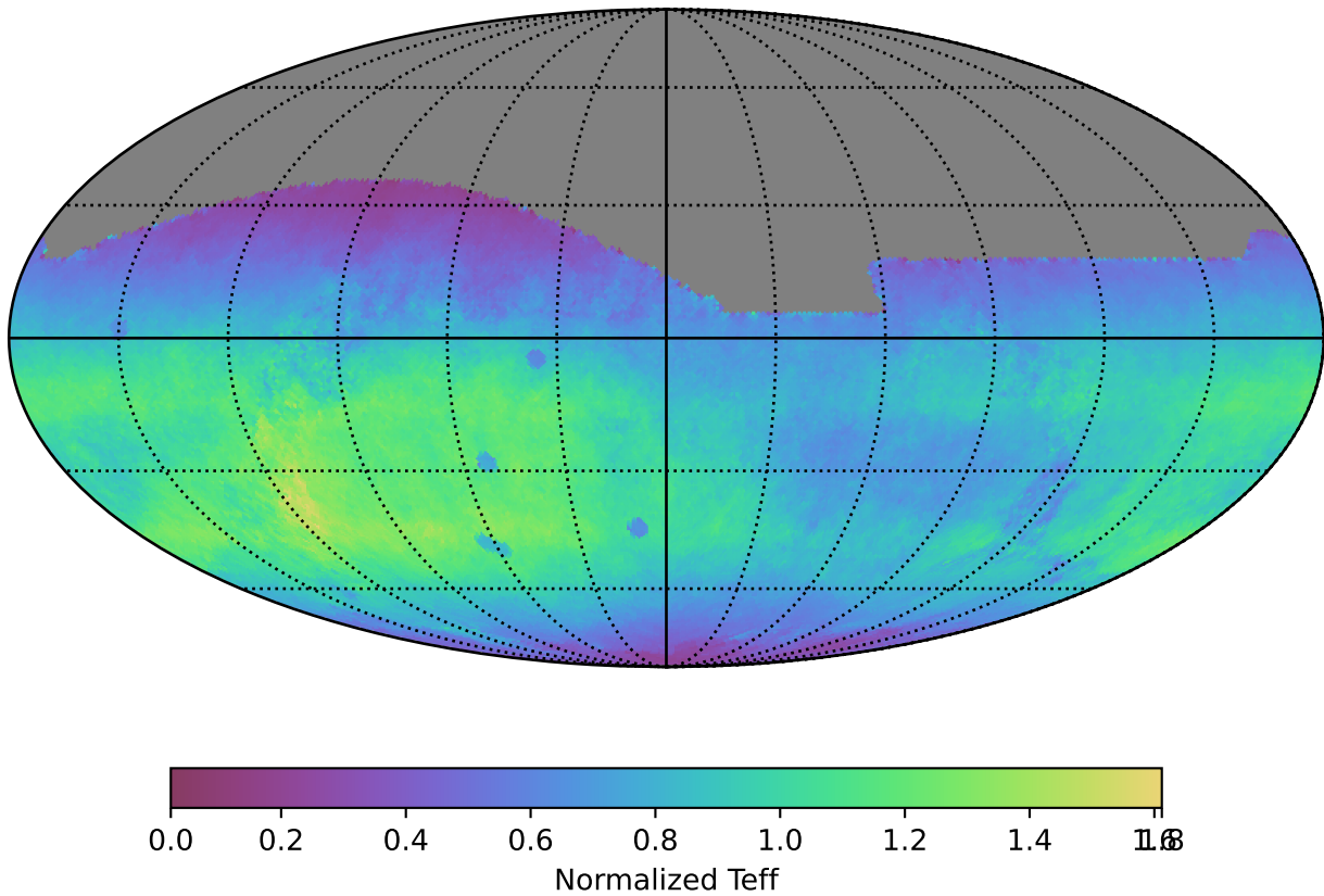
noroll_mjdp365_v3.4_10yrs All sky r band: Normalized Teff
