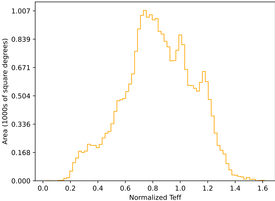
noroll_mjdp365_v3.4_10yrs All sky r band: Normalized Teff
