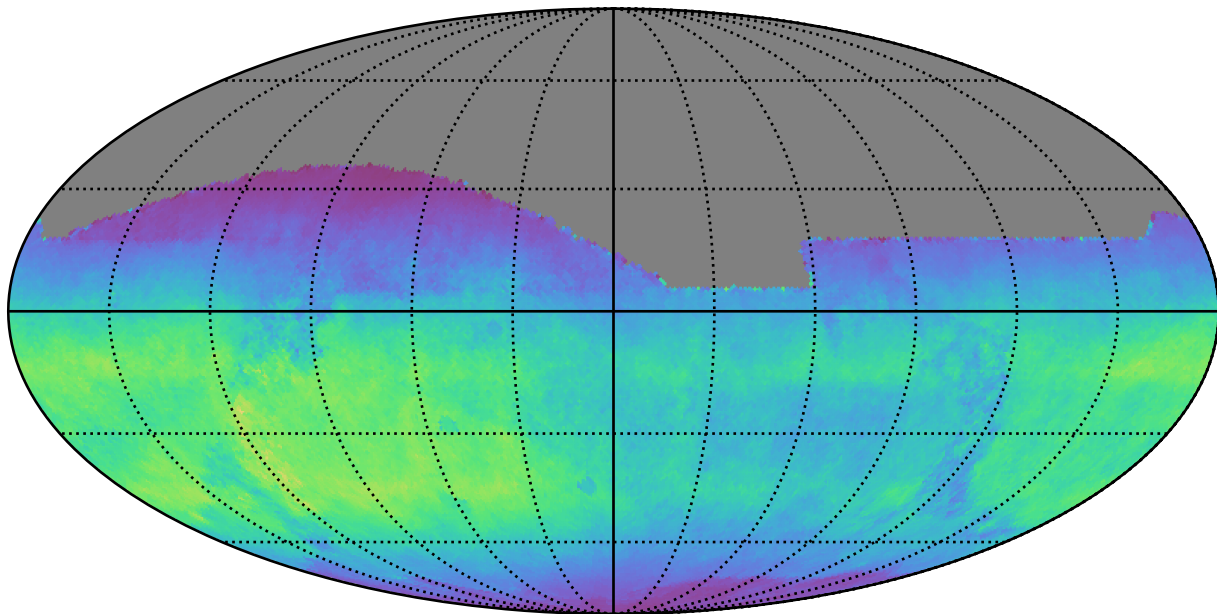
noroll_mjdp365_v3.4_10yrs All sky i band: Normalized Teff
