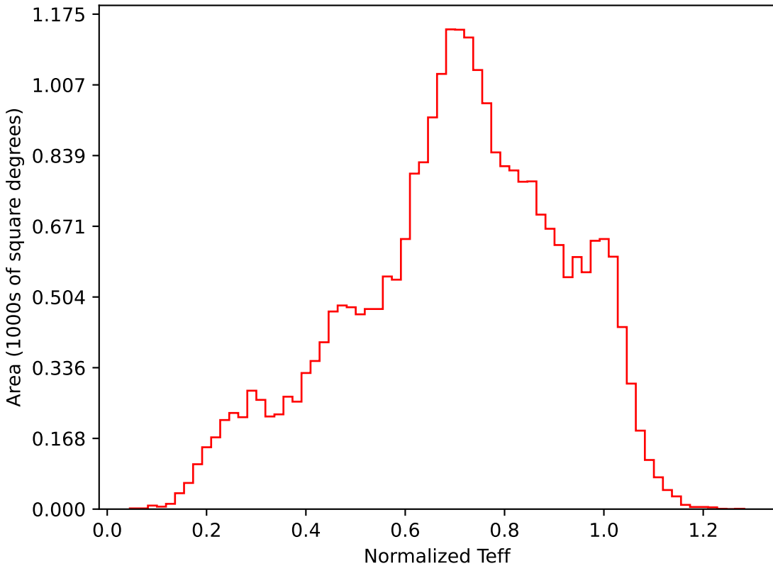
noroll_mjdp365_v3.4_10yrs All sky i band: Normalized Teff
