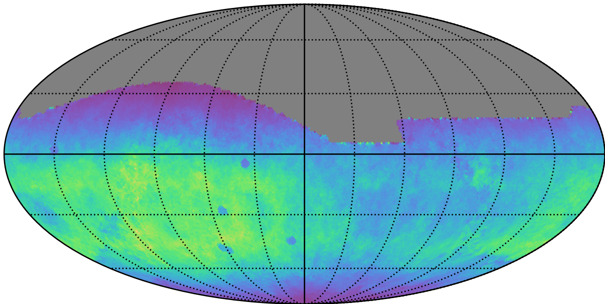
noroll_mjdp365_v3.4_10yrs All sky g band: Normalized Teff
