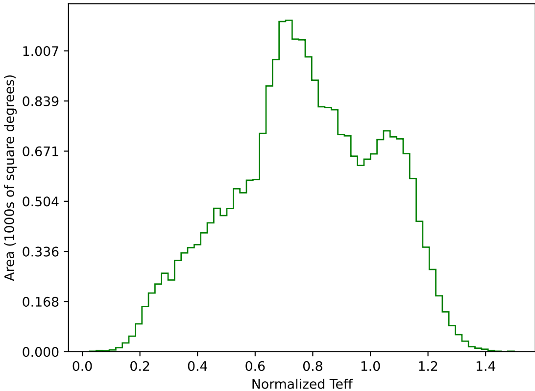
noroll_mjdp365_v3.4_10yrs All sky g band: Normalized Teff
