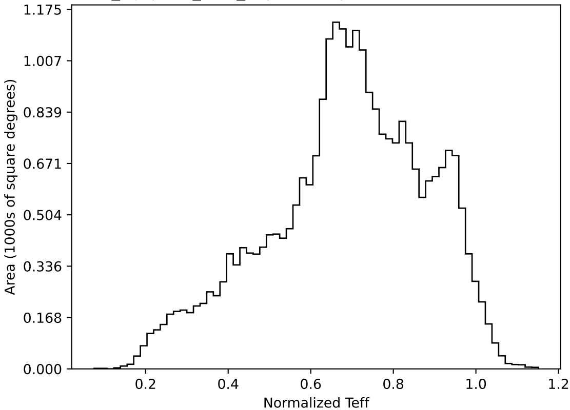
noroll_mjdp365_v3.4_10yrs All sky all bands: Normalized Teff
