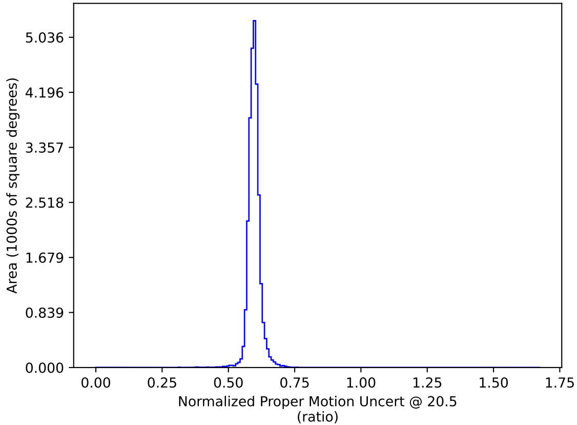
noroll_mjdp365_v3.4_10yrs All sky: Normalized Proper Motion Uncert @ 20.5
