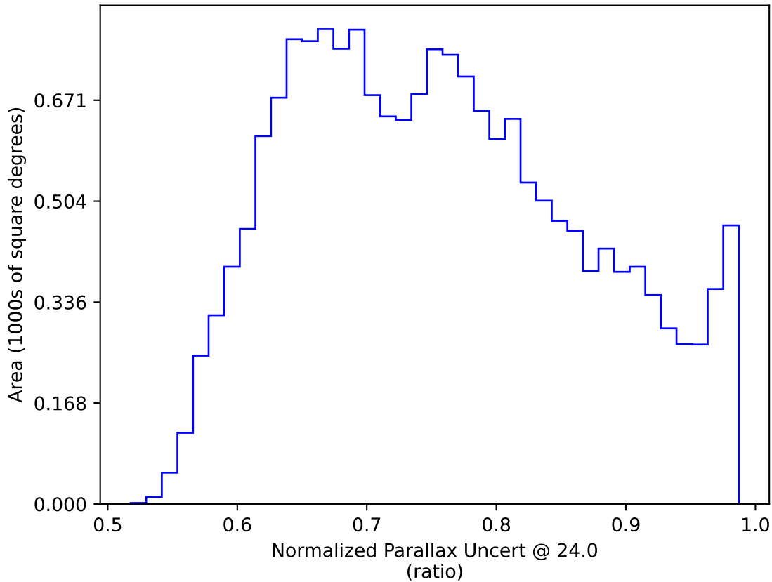
noroll_mjdp365_v3.4_10yrs WFD: Normalized Parallax Uncert @ 24.0
