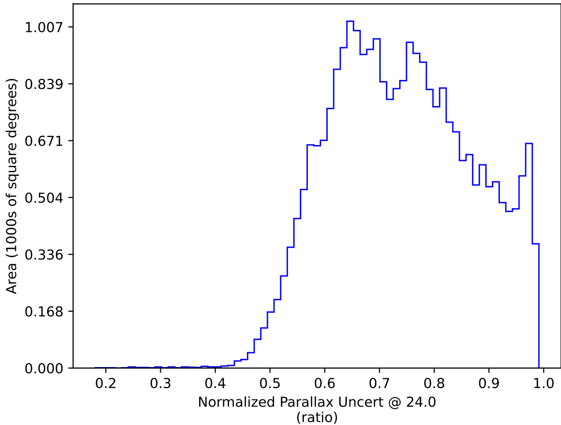
noroll_mjdp365_v3.4_10yrs All sky: Normalized Parallax Uncert @ 24.0
