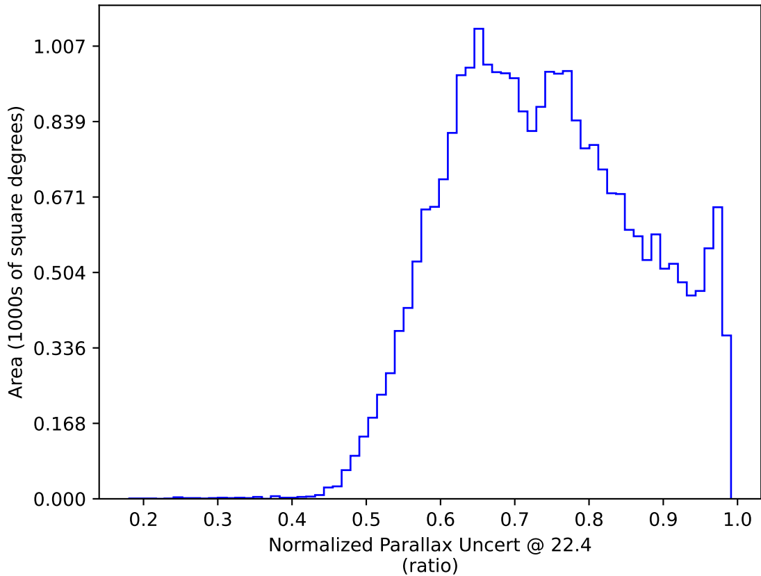
noroll_mjdp365_v3.4_10yrs All sky: Normalized Parallax Uncert @ 22.4
