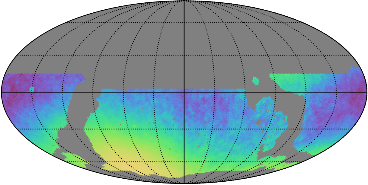
noroll_mjdp365_v3.4_10yrs WFD y band only: Normalized Parallax Uncert @ 21.3
