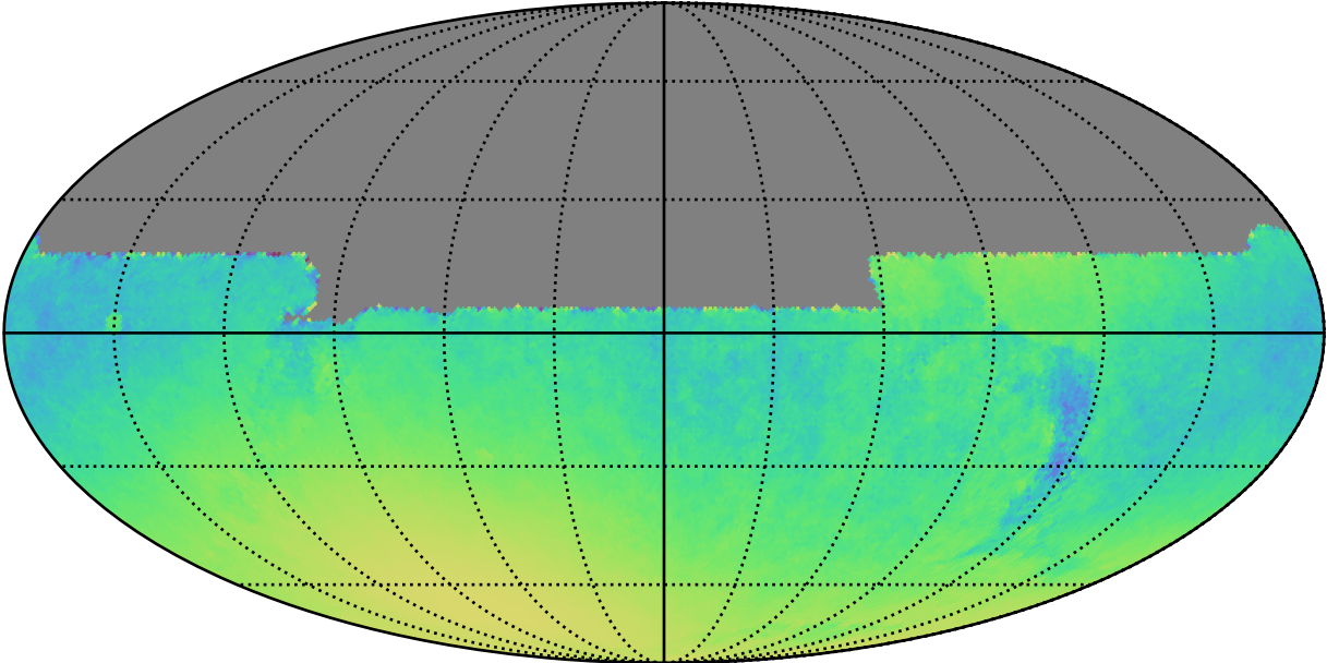
noroll_mjdp365_v3.4_10yrs All sky y band only: Normalized Parallax Uncert @ 21.3
