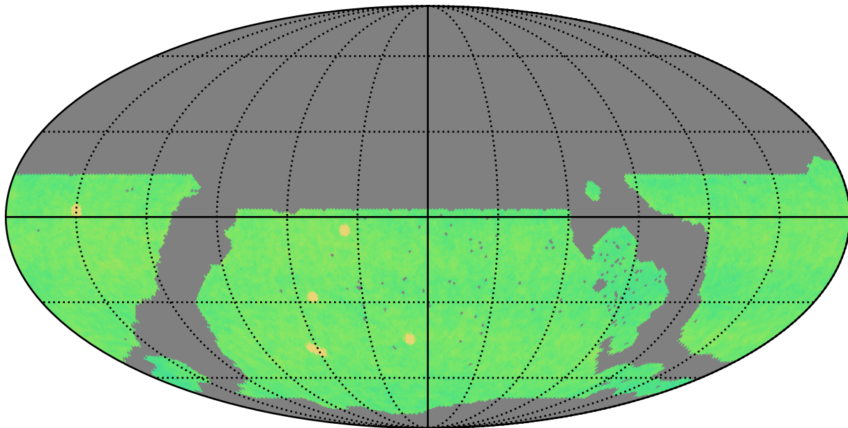
noroll_mjdp365_v3.4_10yrs WFD all bands: N Unique Nights
