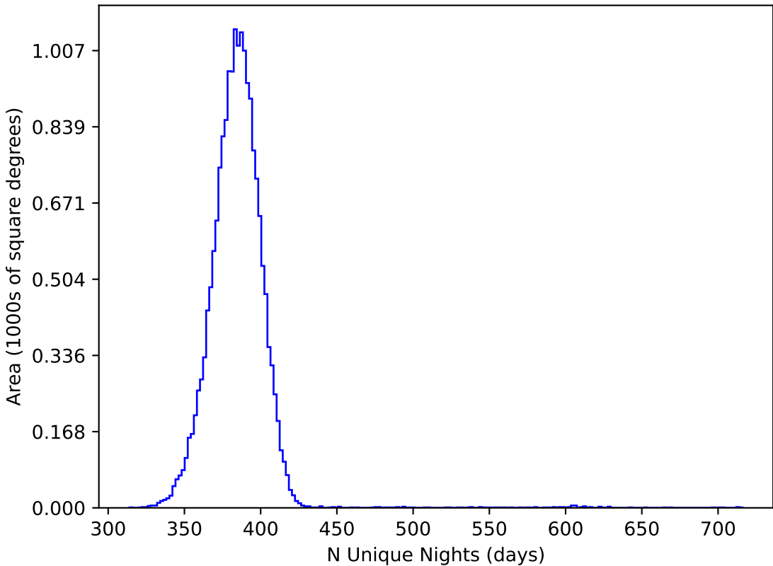
noroll_mjdp365_v3.4_10yrs WFD all bands: N Unique Nights
