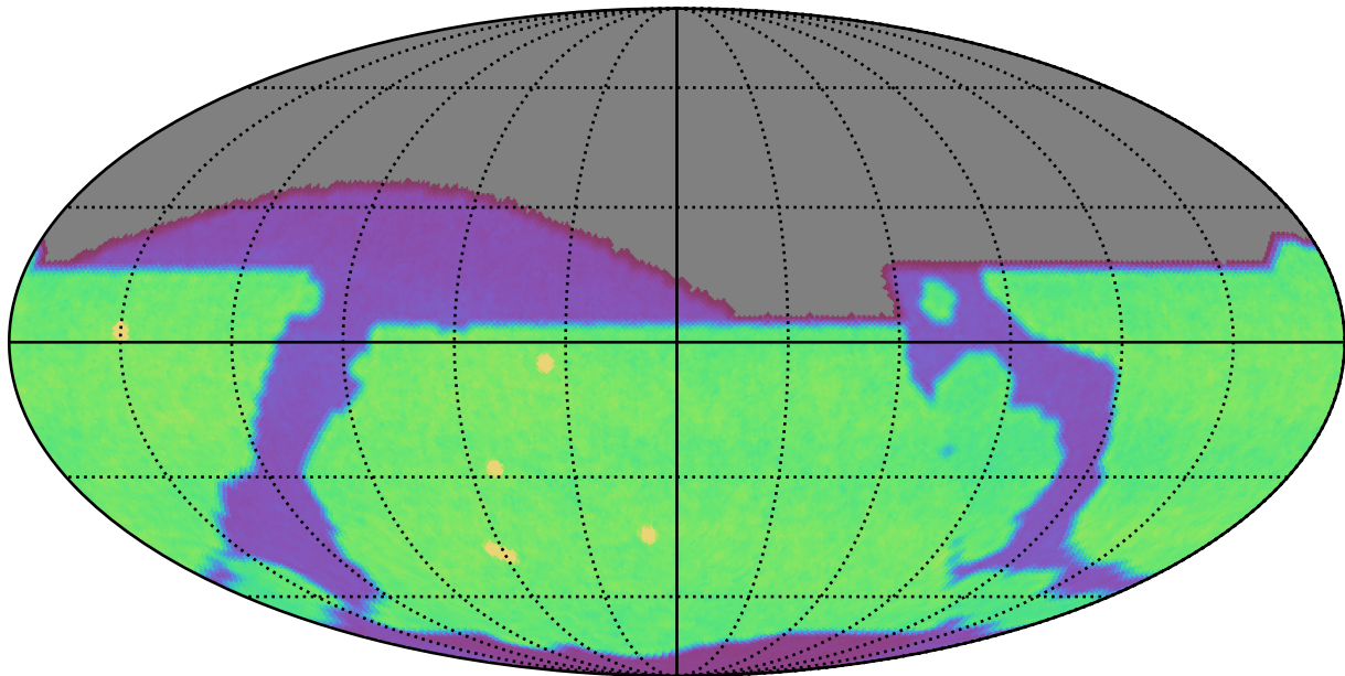
noroll_mjdp365_v3.4_10yrs All sky all bands: N Unique Nights
