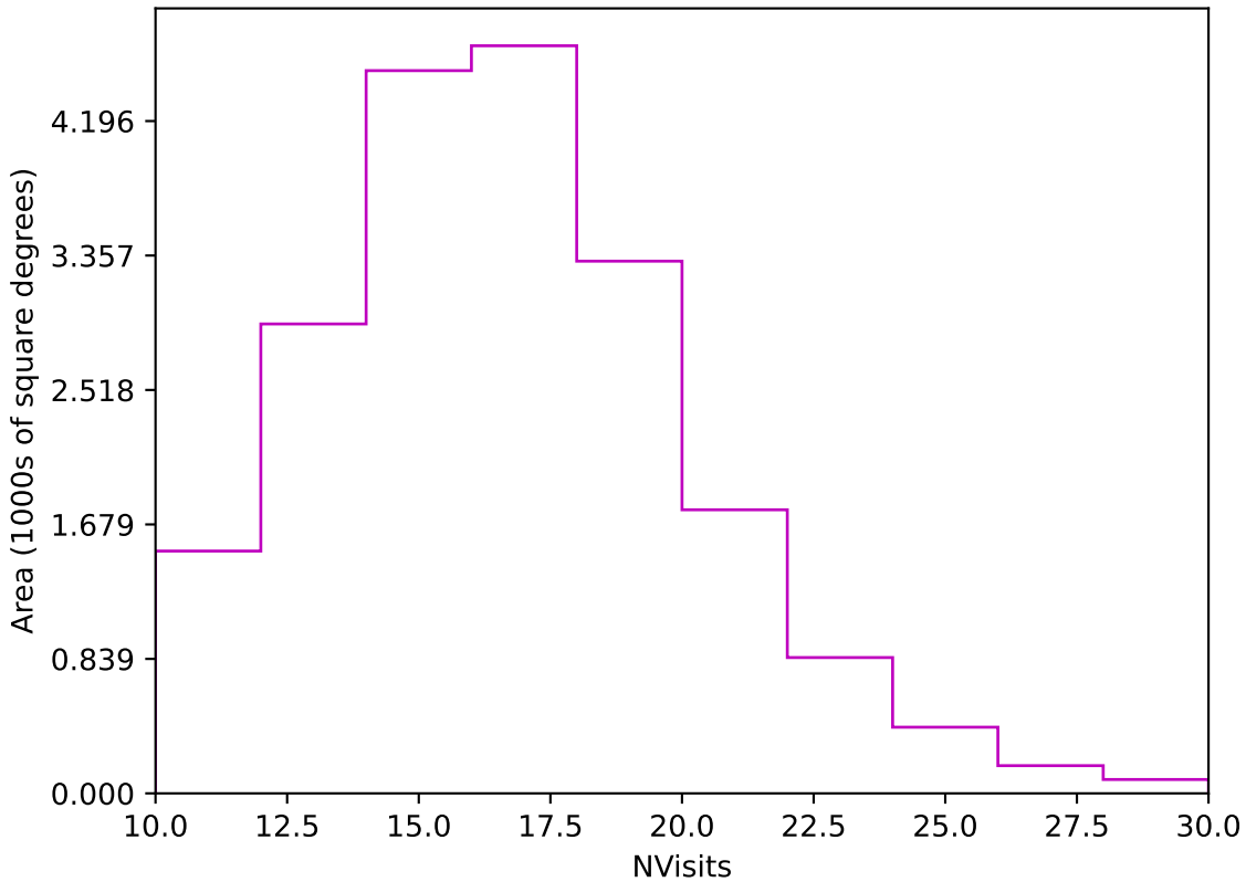
noroll_mjdp365_v3.4_10yrs Yr 3-4 z band: NVisits
