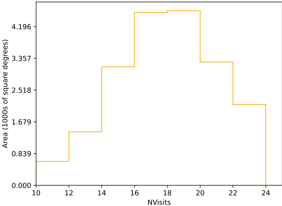
noroll_mjdp365_v3.4_10yrs Yr 3-4 r band: NVisits
