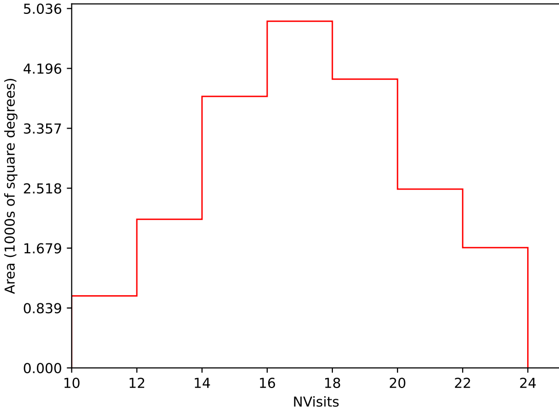
noroll_mjdp365_v3.4_10yrs Yr 3-4 i band: NVisits
