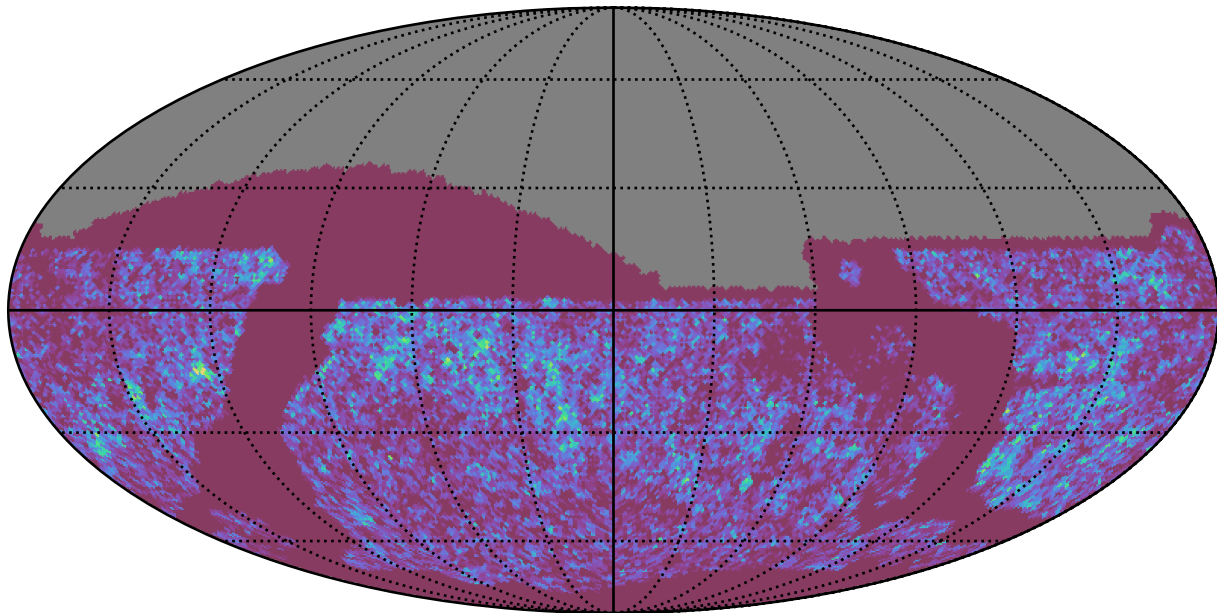
noroll_mjdp365_v3.4_10yrs Yr 3-4 all bands: NVisits
