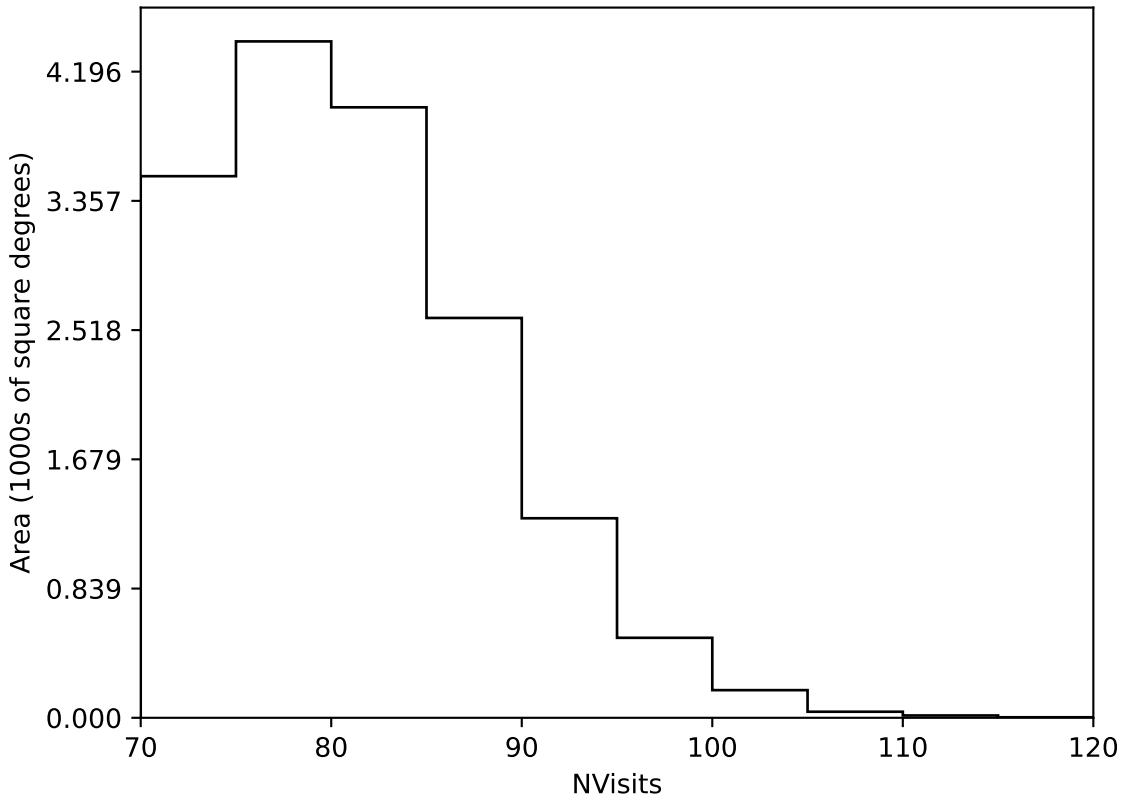
noroll_mjdp365_v3.4_10yrs Yr 3-4 all bands: NVisits
