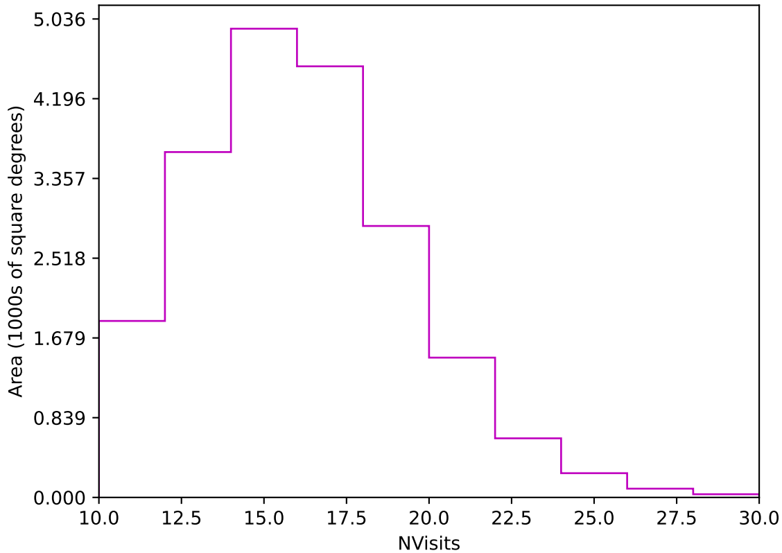
noroll_mjdp365_v3.4_10yrs Yr 1 z band: NVisits
