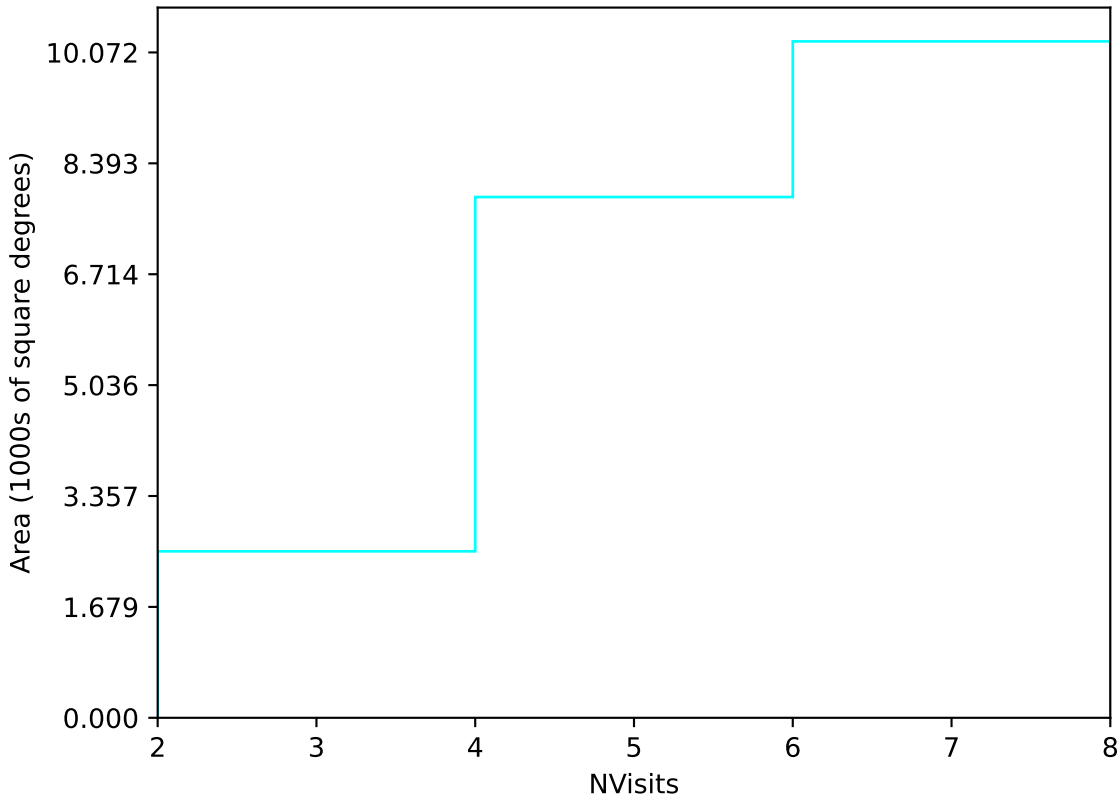
noroll_mjdp365_v3.4_10yrs Yr 1 u band: NVisits
