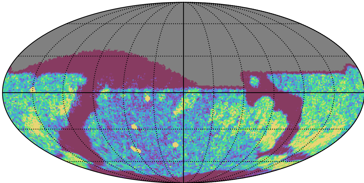
noroll_mjdp365_v3.4_10yrs Yr 1 r band: NVisits
