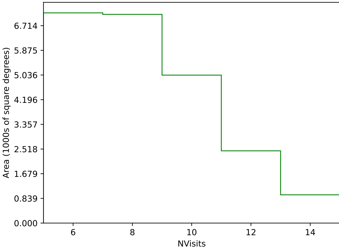
noroll_mjdp365_v3.4_10yrs Yr 1 g band: NVisits
