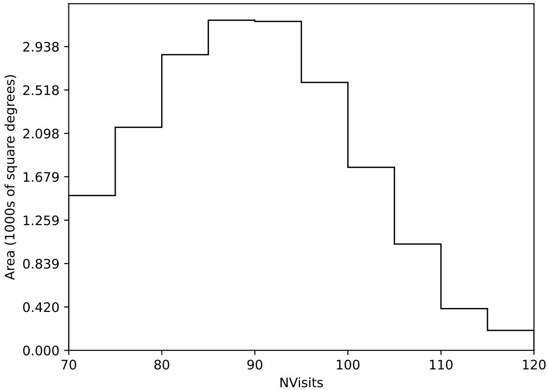
noroll_mjdp365_v3.4_10yrs Yr 1 all bands: NVisits
