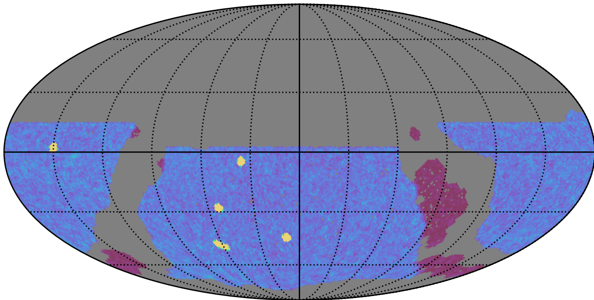
noroll_mjdp365_v3.4_10yrs WFD y band: NVisits
